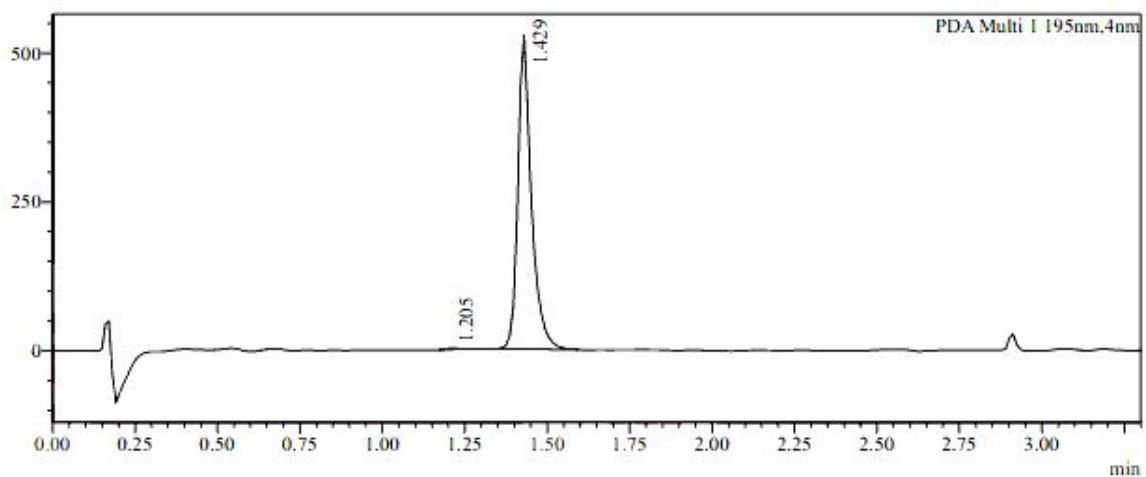
Chromatogram mAU
