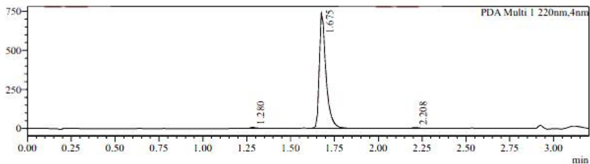
MS Chromatogram
